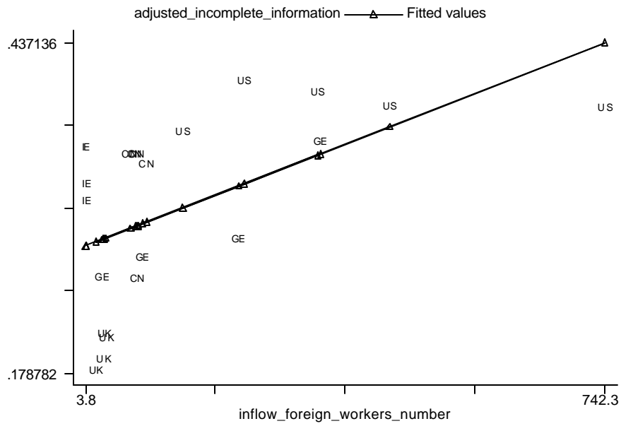
Figure 5: Adjusted Incomplete Information versus Inflow of Foreign Workers (in number).
